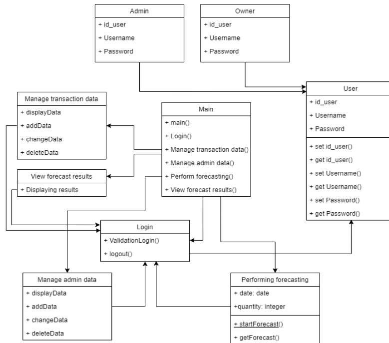
Figure 2. Class diagram
